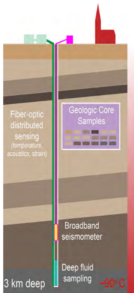
Schematic of pilot borehole.
